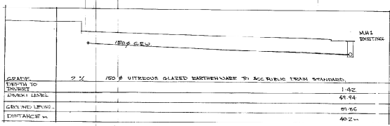
SEWER CONNECTION - LONG SECTION Scale: Horizontal 1:200, Vertical 1:100
