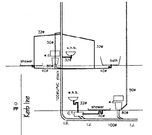
PLUMBING SCHEMATIC
