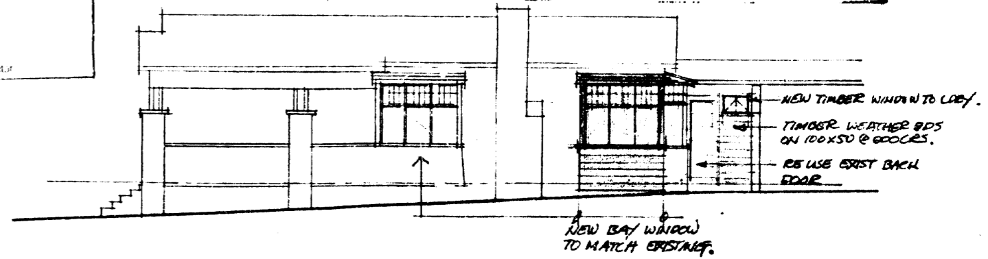
EAST ELEVATION 1:100
