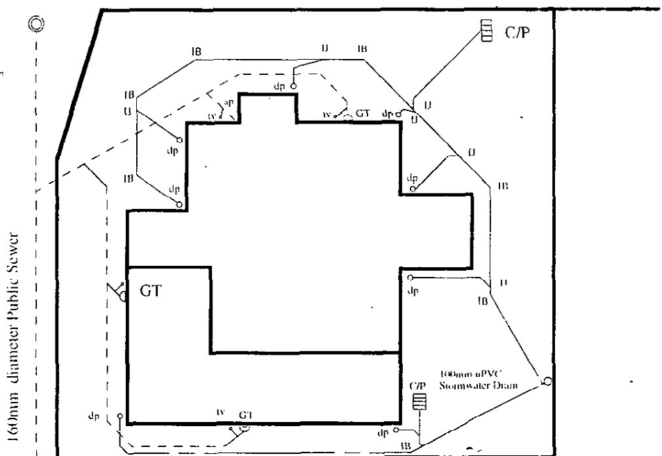
Lot 17 GOODLAND St. EPSOM Scale 1:200
